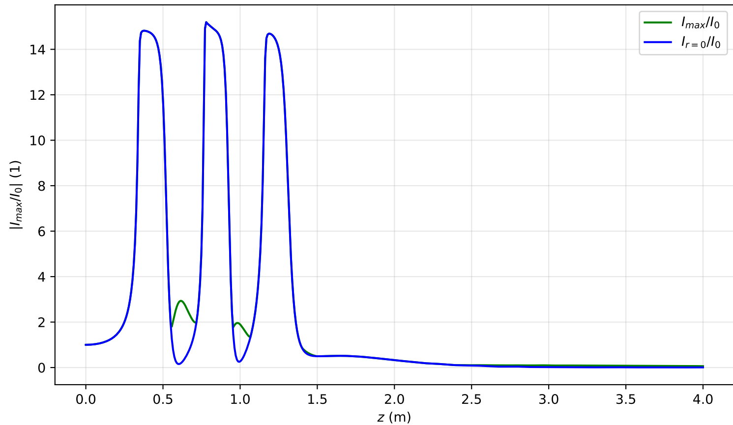
I_{\max}(x = 0, y = 0, z)/I_0 , \text{Pin}=7.5\text{Pcr} , artificial time
